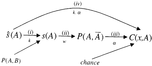
FIG. 1. A schematic representation of the relationship between variables. Note that \hat{s}(A) refers to assessed strength of evidence for hypothesis A ; s(A) refers to hypothetical support for hypothesis A ; P(A, \bar{A}) refers to judged probability of hypothesis A against its complement; C(x, A) refers to the certainty equivalent for the prospect that pays \$x if and only if hypothesis A obtains; P(A, B) refers to the judged probability of hypothesis A against hypothesis B , assuming either A or B obtains (but not both); and chance refers to choices between chance prospects that are used to parameterize the utility function for monetary gains. The parameters k (the strength-support scaling parameter), w (the global weight for discounting support of alternative hypotheses), and \alpha (the utility function parameter), listed below the arrows, are required to estimate the variable to the right of the corresponding arrow from the variable to the left of that arrow.
